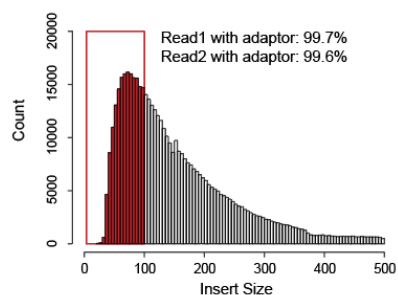
Ligation Test 1 Insert Size Histogram
