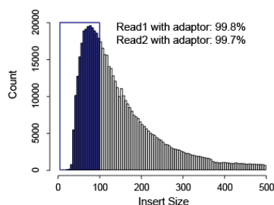
Ligation Test 2 Insert Size Histogram
